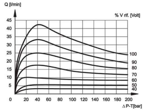
SPOOL TYPE C26
