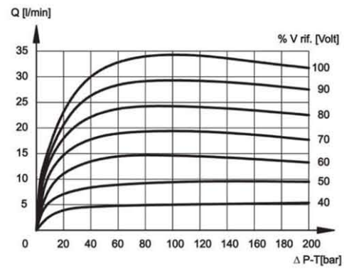
SPOOL TYPE A16
