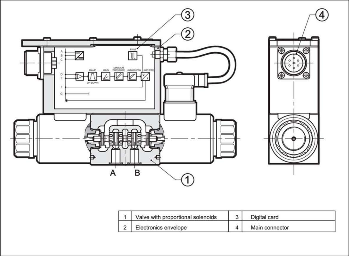
5.2 - Functional block diagram
