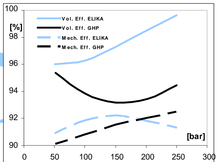
Efficiency pump comparison [%] Marzocchi GHP2 – ELIKA ELI 2, same displacement 17.8 cm 3 /rev.
