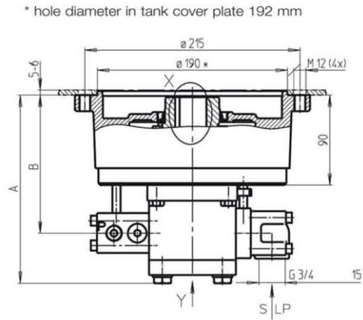
Dimension drawing 2
