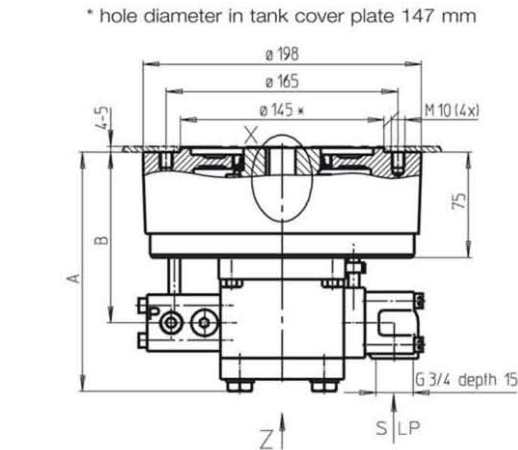
Dimension drawing 1
