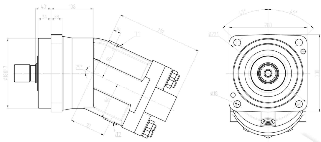
T1, T2 - case drain ports M22x1,5-18 ISO 6149-1
